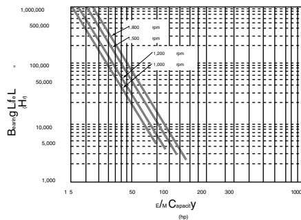
Bearing Life
