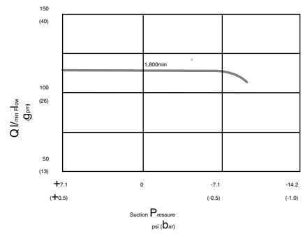
Self-Priming Capability
