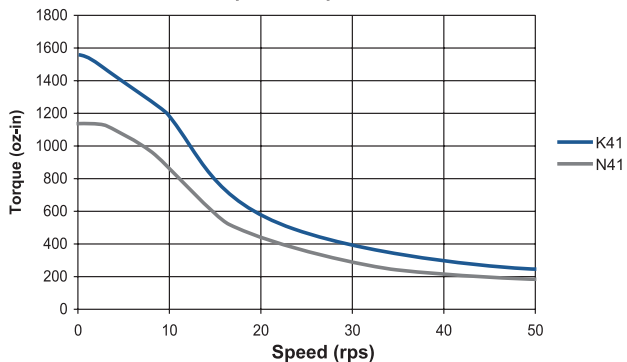
Speed Torque N, K 41
