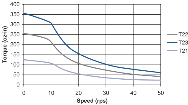
Speed Torque N, K 31
